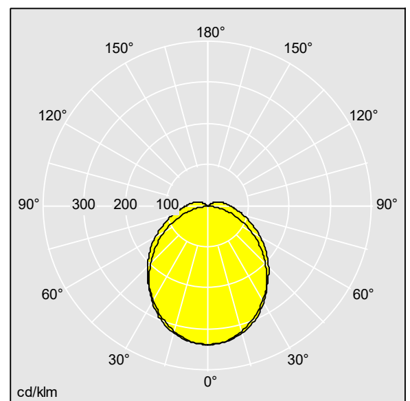
D45933_AQFPRO_L_6400-840_PC_MB_HF.Idt
