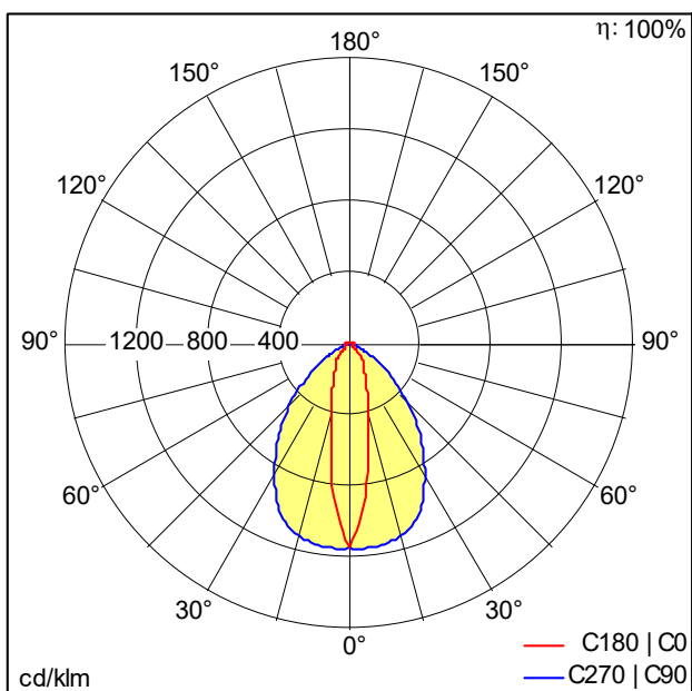
D45916_AMP_L_8000-840_CH_NB_LDO.idt
