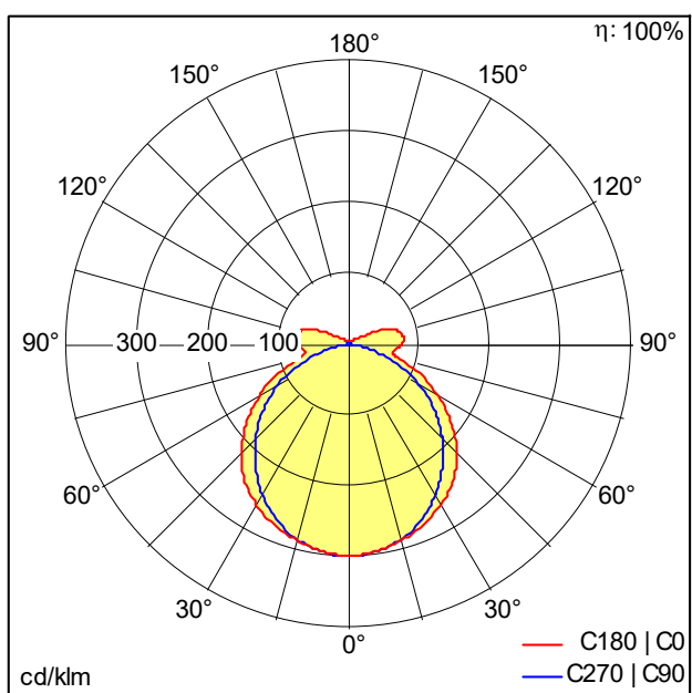
D45913_AMP_L_BAS_6400-840_CH_MB_LDO.idt
