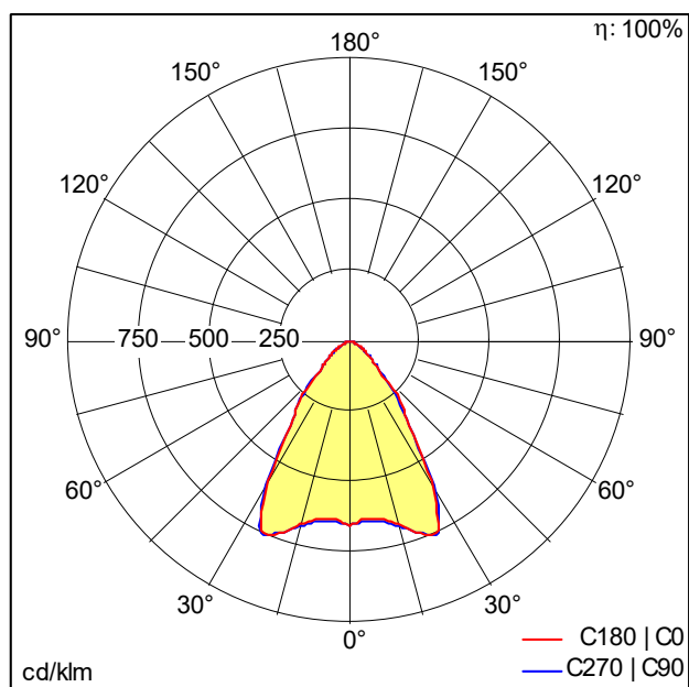
D42326AA_TECTON_MIREL_LED2700-840_L1000_LDO_BK.Idt
