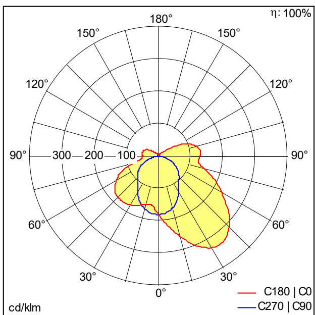
D45909_AMP_L_4000-840_PC_AB_LDO.Idt
