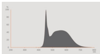
EPREL data spectral diagram PROF LED r 6500K
