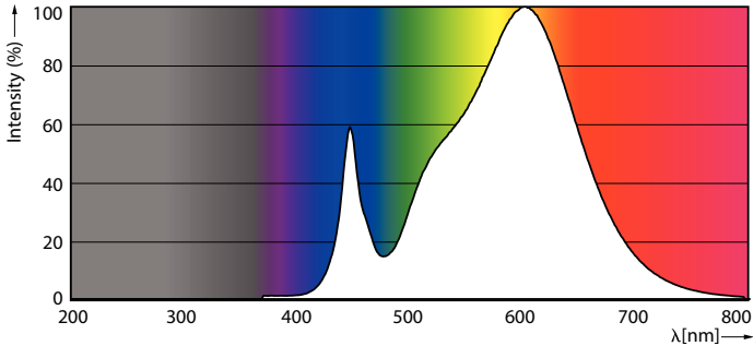
Spectral Power Distribution Colour – MAS LEDtube VLE 1200mm 13.1W/15.5W 830T8
