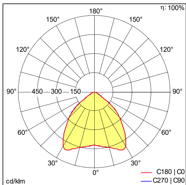
D43022 MIRL LAY 3800-830 M625L WB EVG WH.Idt
