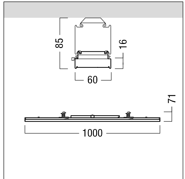
ZS_TEC_M_C_LED_Balken_L1000.wmf
