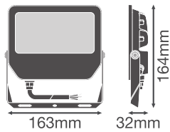
FL COMP 30/50 V 42W ML8304065
