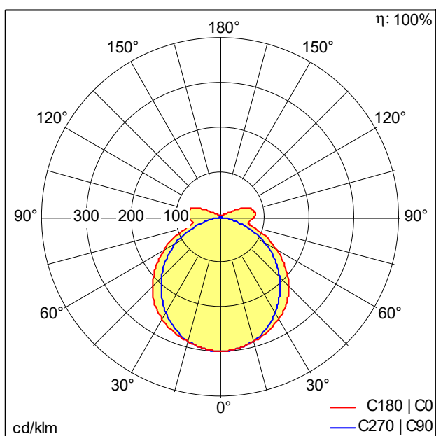
D45913_AMP_L_BAS_6400-840_CH_MB_LDO.idt
