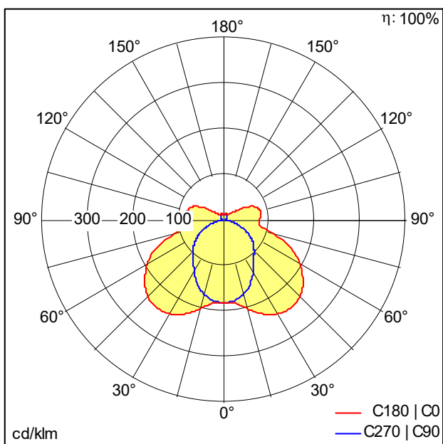
D45887_AMP_S_4600-840_PC_WB_LDO.idt
