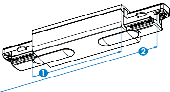
Middle feed GB 14 1. 80 mm, 2. 145 mm
