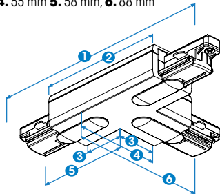
T-feed GB 36, 37, 39, 40 1. 145 mm, 2. 80 mm, 3. 25 mm, 4. 55 mm, 5. 58 mm, 6. 88 mm
