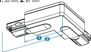
L-feed GB 34, 35 1. 55 mm, 2. 87 mm
