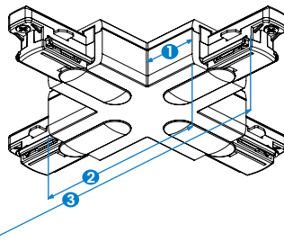
Middle feed GB 14 1. 80 mm, 2. 145 mm
