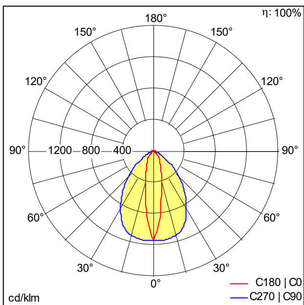
D45911_AMP_L_8000-840_PC_NB_LDO.Idt
