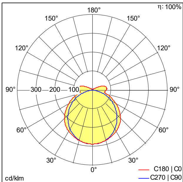
D45903_AMP_L_6400-840_PM_MB_LDO.idt
