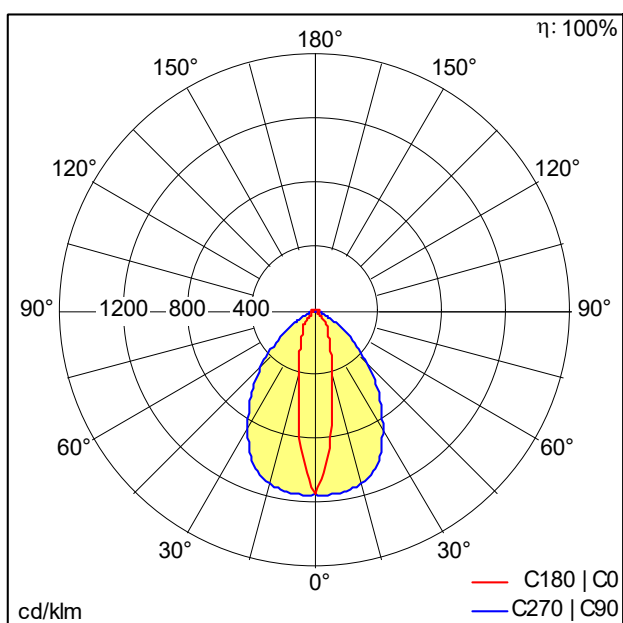
D45916_AMP_L_LT_8000-840_CH_NB_IVG.idt
