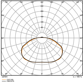
MAG LED RING P 12W ML 840 AC
