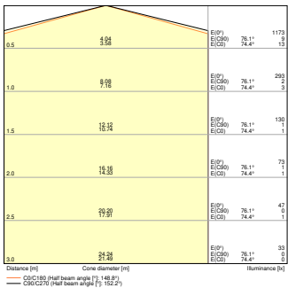
MAG LED RING P 12W ML 830 AC
