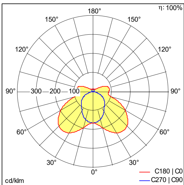
D45907_AMP_L_8000-840_PC_WB_LDO.idt
