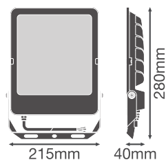
FL COMP 125/150 V 105W ML8304065
