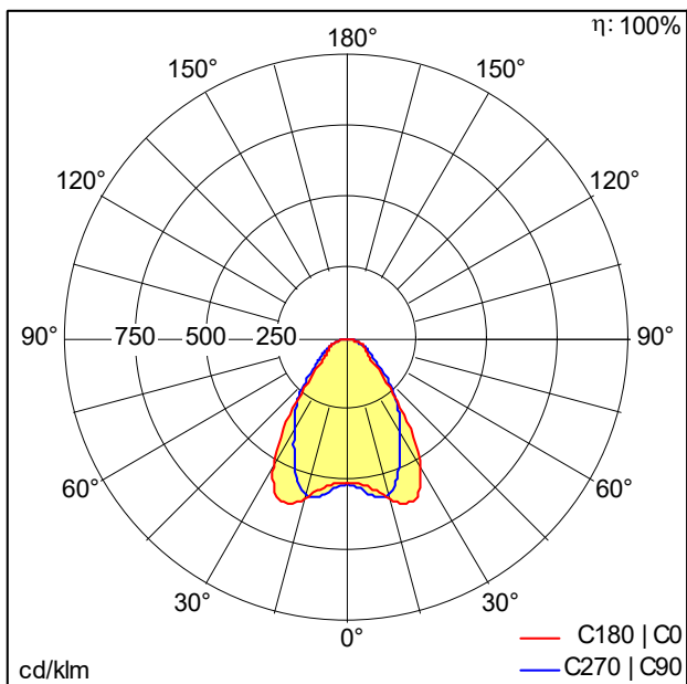
D35001_TECTON_C_5500-840_L1500_WB_EVG_WH.Idt
