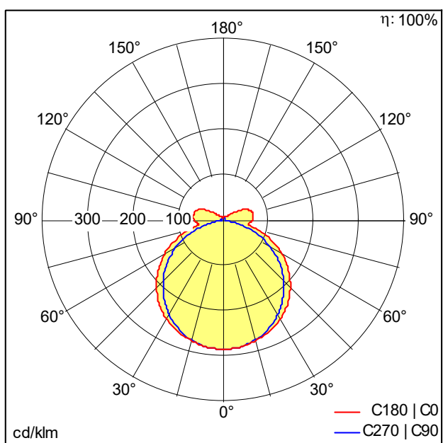
D45888_AMP_S_4600-840_PC_MB_LDO.idt
