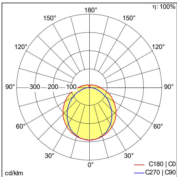
D44081AA_TECTON_B_BASIC_LED5200-840_L1522_LDE_SR.Idt
