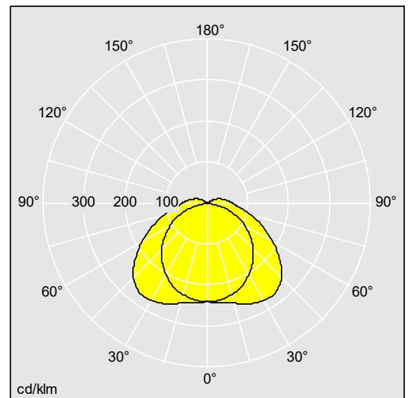
D45932_AQFPRO_L_6400-840_PC_WB_HFI.ltd
