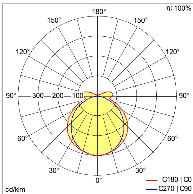
D45913_AMP_L_8000-840_CH_MB_LDO.Idt
