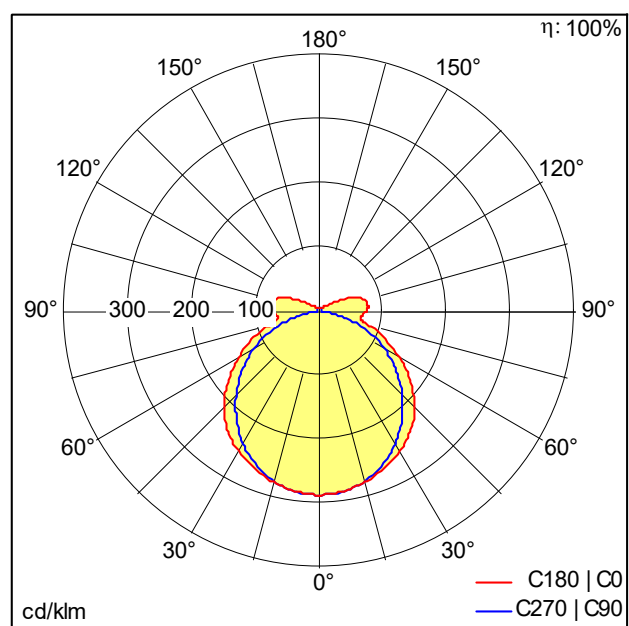
D45903_AMP_L_BAS_6400-830_PM_MB_EVG.Idt
