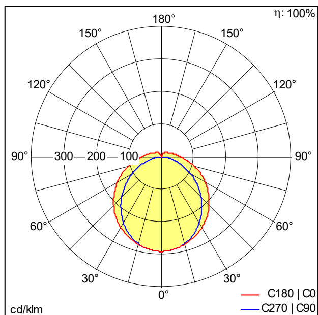
D44080AA_TECTON_B_BASIC_LED8000-840_L1522_EVG_WH.Idt
